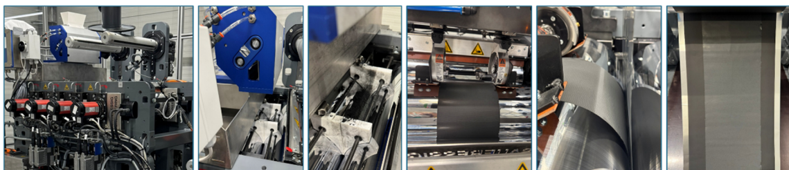
Figure 18: Images taken during the dosing process with the roller feeder from Coperion K-Tron, as well as during the film formation and lamination process with the ProLiT calender from Saueressig/ Matthews Engineering (created by M. Nickl)
