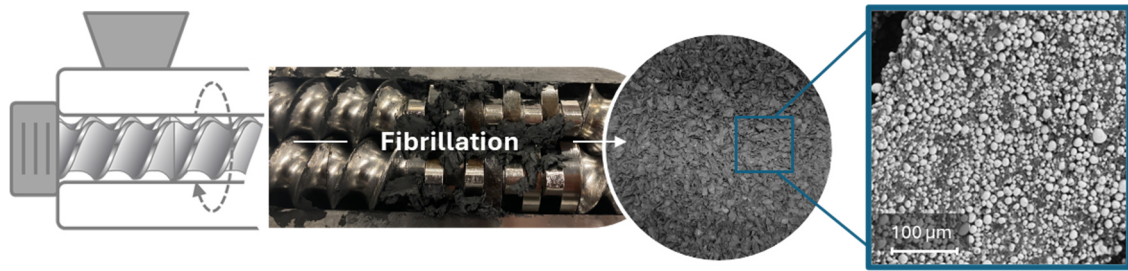
Figure 17: Schematic of a batch mixing process in an extruder with resulting fibril morphology (created by M. Nickl).
